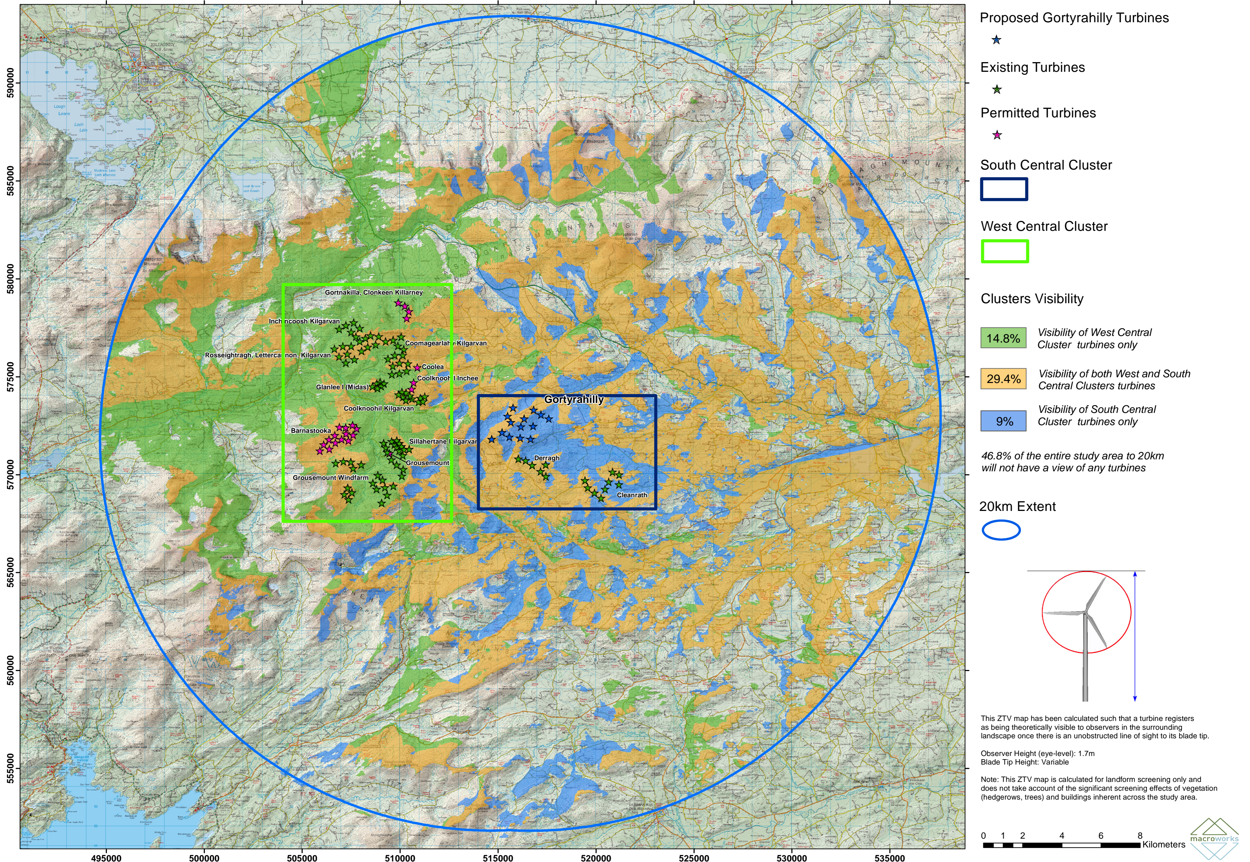
Figure 12.8 Delta ZTV indicating the theoretical visibility of the central wind farm clusters within the proposed Gortyrähilly Wind Farm study area
